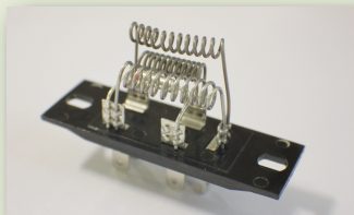
GE's Item Code : 2331-05 4 Speed Resistor Blower
